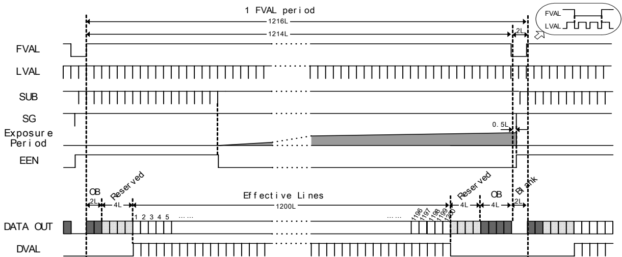
Fig. 16. Vertical timing
